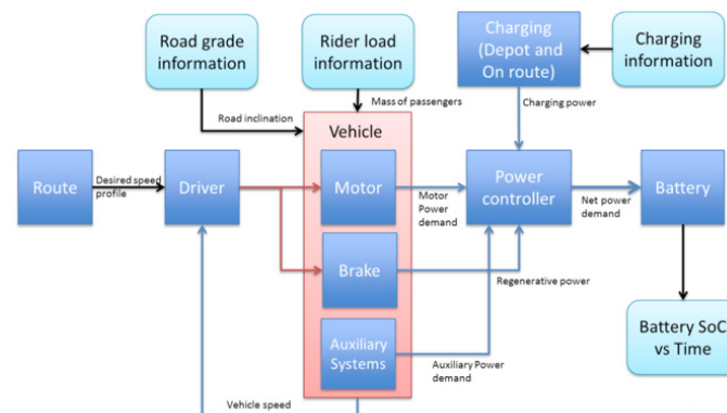
The model structure includes input from a variety of sources, and captures the dynamics of a range of components in a typical electric bus transit environment.
