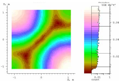
Figure 7: CIE color difference analysis calculates and optimizes system color performance. This is useful for producing an even color distribution.
