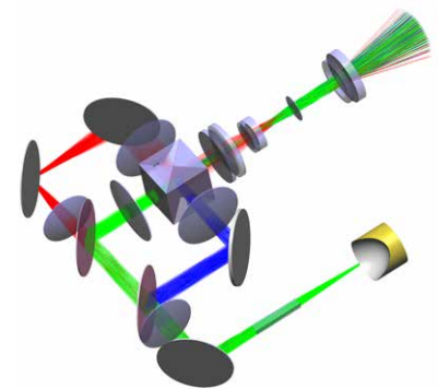
Figure 1: LightTools' smart modeling capabilities make it easy to quickly build complex illumination systems. Point-and-shoot ray tracing provides instant feedback on system alignment.
