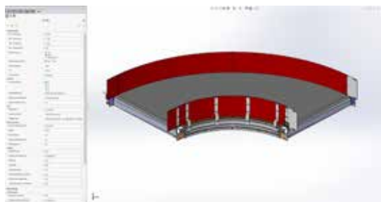
“Preconfiguring” a curved belt conveyor with Tacton Design Automation. The user interface for entering the individual parameters is visible on the left side of the screen.
