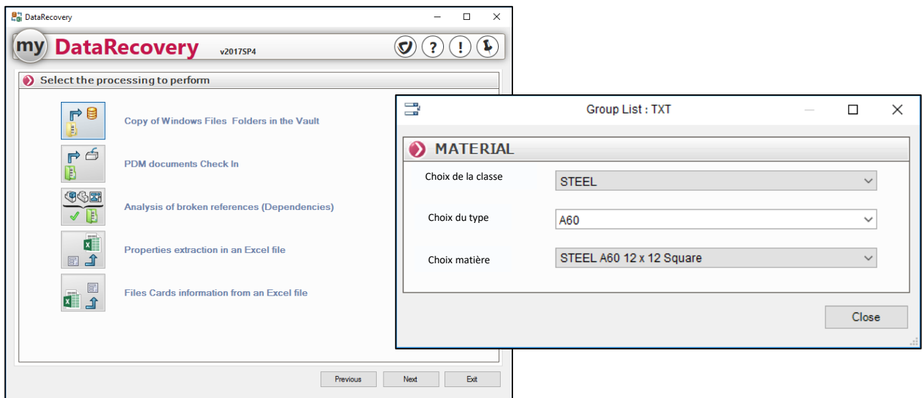
DataRecovery & DynamicList
